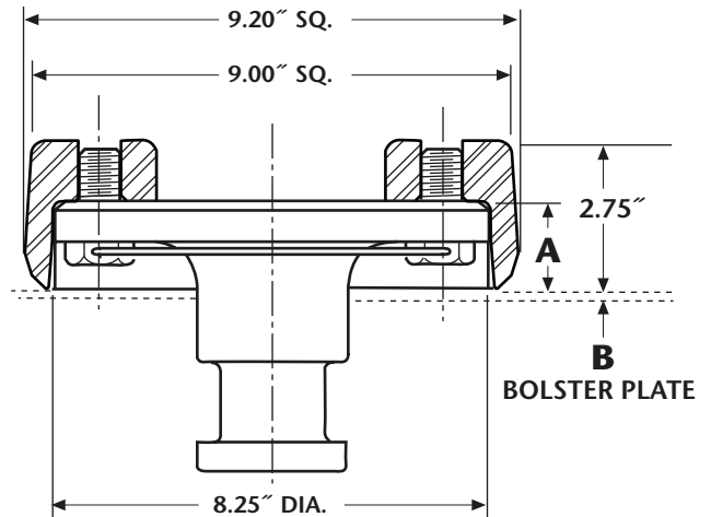
SAE 2.00" KING PIN
