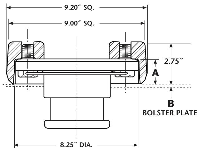
SAE 3.50" KING PIN
