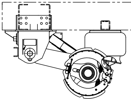
CBX TOP MOUNT
