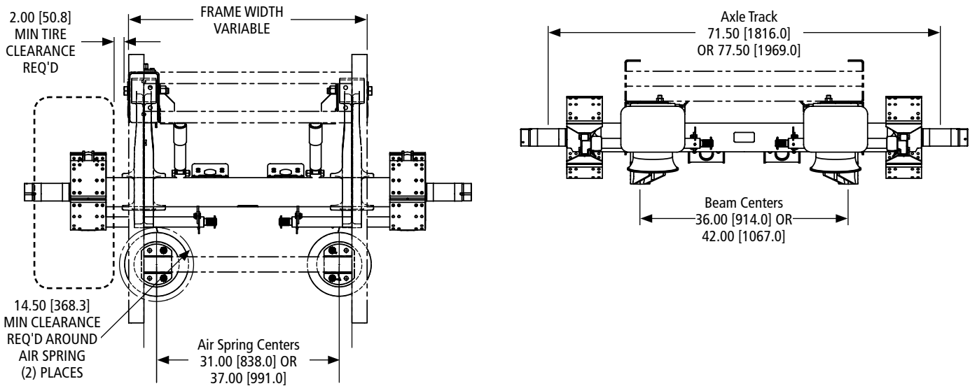
CBX25U (with parallel spindle drum brakes shown) All Dimensions Are Reference
