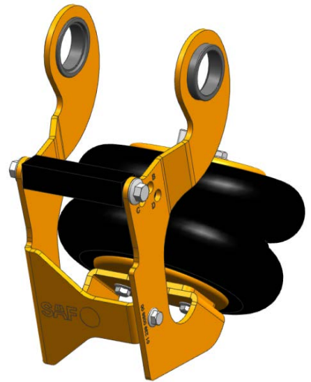
Illustration of axle lift - 03 027 1278 01
