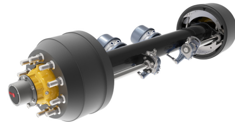
SC5 DRUM BRAKE AXLE
