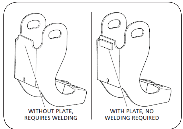
Figure 1 - New bolt-on bracket
