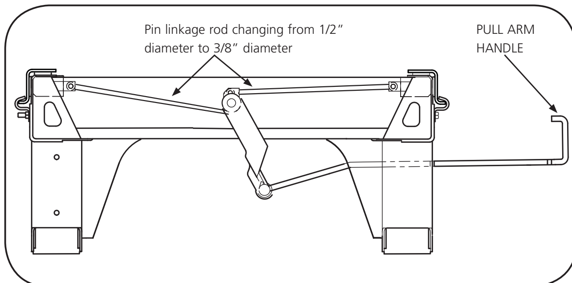
Figure 1 - Pin Linkage Rods
