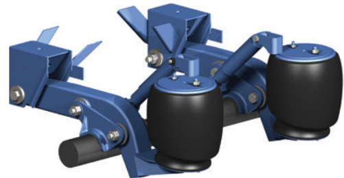
RL Trailer Air Suspension Models
